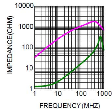
CHOK3216S102T
