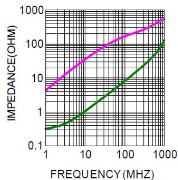
CHOK3216S601T
