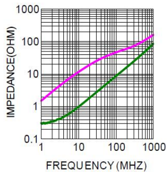
CHOK3216S221T
