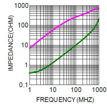
CHOK3216S222T
