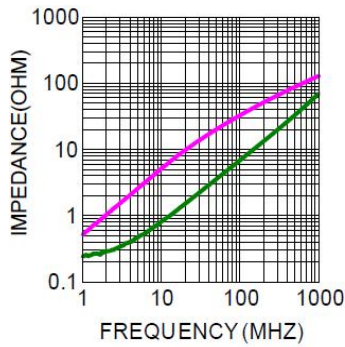
CHOK3216S161T
