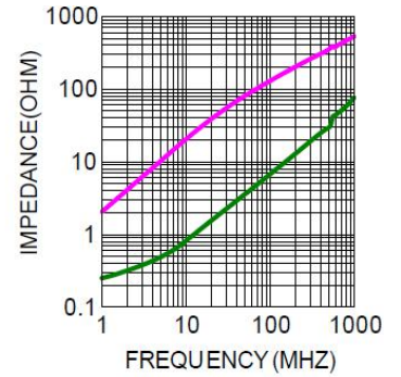
CHOK3216S501T
