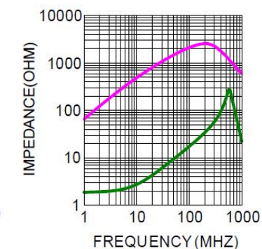
CHOK3216S222T
