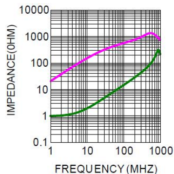
CHOK3216S601T
